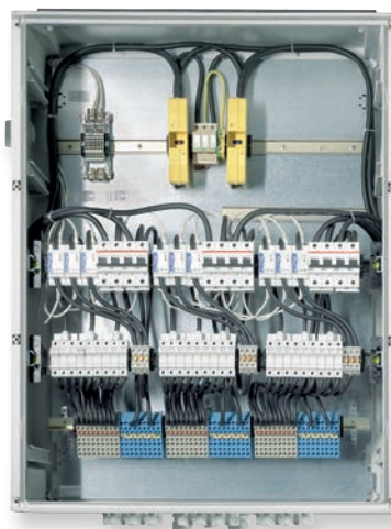
DC combiner box
