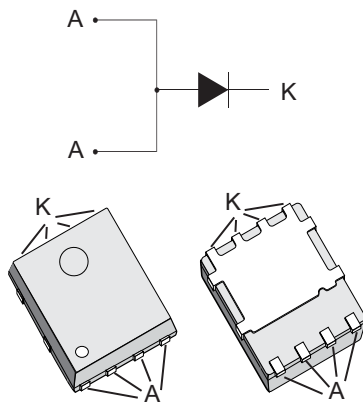
PowerFLAT™ 5x6
