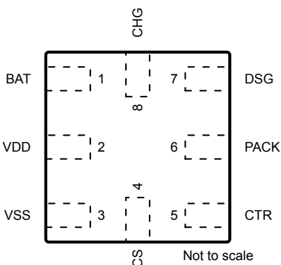
Figure 5-1. RUG Package 8-Pin X2QFN Top View
