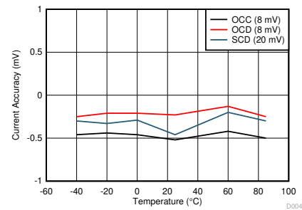
Figure 6-4. Overcurrent Accuracy Across Temperature
