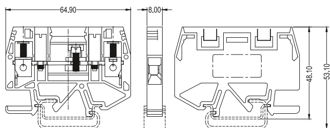
JXB-6S1/35
