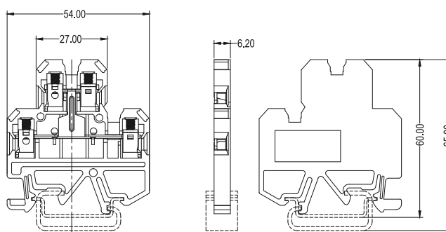
JXB-4/35, JXB-4/35L
