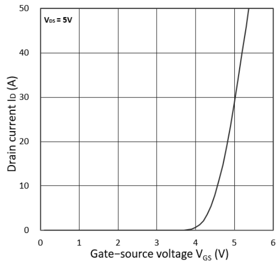
Figure 2. Transfer Characteristics
