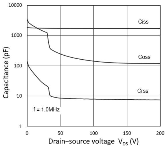
Figure 7. Capacitance Characteristics
