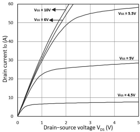
Figure 1. Output Characteristics
