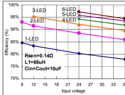
I_{OUT}=700mA
