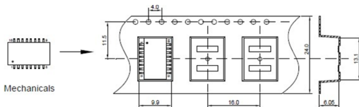
Tape & Reel
