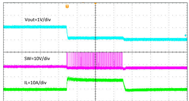
Figure 7-23. TPS566231 Normal Operation to Output Hard Short
