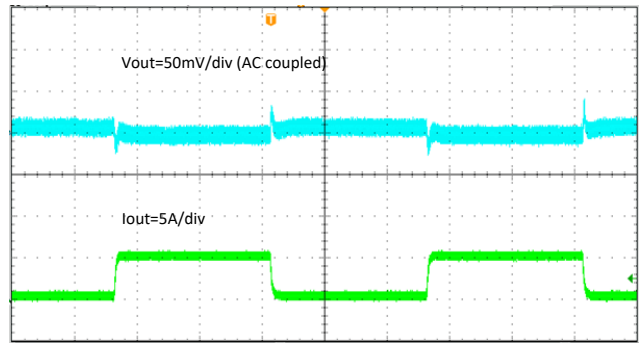
0.6 A to 5.4 A Slew Rate = 2.5 A/ \mu s Figure 7-21. TPS566238 Transient Response
