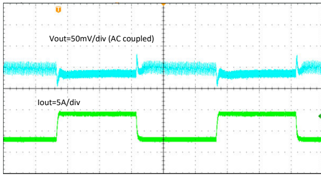
0.1 A to 6 A Slew Rate = 2.5 A/ \mu s Figure 7-20. TPS566231 Transient Response
