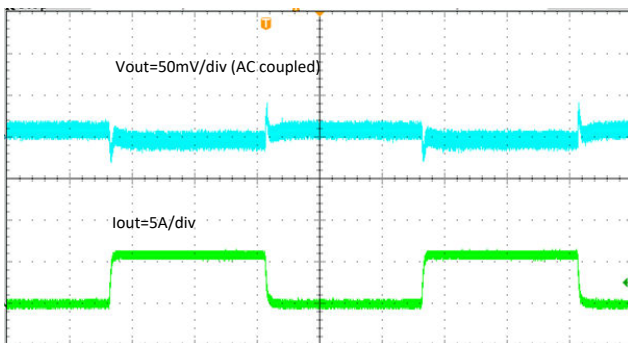
0.1 A to 6 A Slew Rate = 2.5 A/ \mu s Figure 7-22. TPS566238 Transient Response
