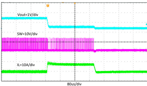
Figure 7-24. TPS566238 Normal Operation to Output Hard Short
