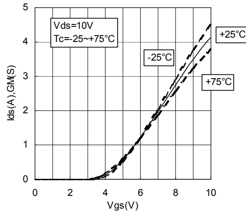
Vgs-Ids CHARACTERISTICS 2
