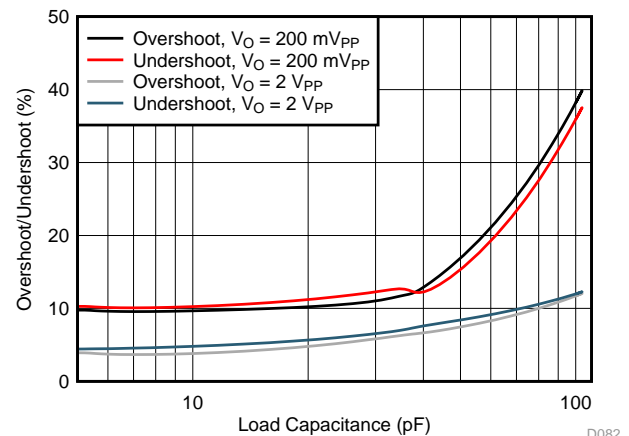
See Figure 65, Gain = 1 V/V, R_F = 0\ \Omega
