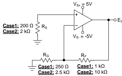
Figure 73. Comparing Noise Contributors for Two Cases With the Amplifier in a Noninverting Gain of 5 V/V
