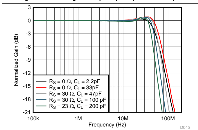
See Figure 65 and Figure 63, V_O = 20\text{ mV}_{PP} , Gain = 2 V/V
