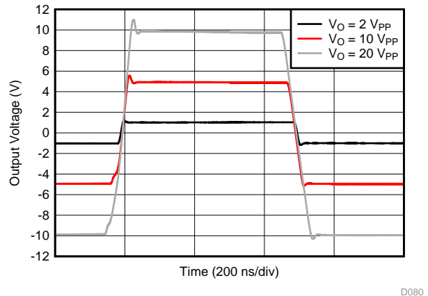
See Figure 65, Gain = 2 V/V
