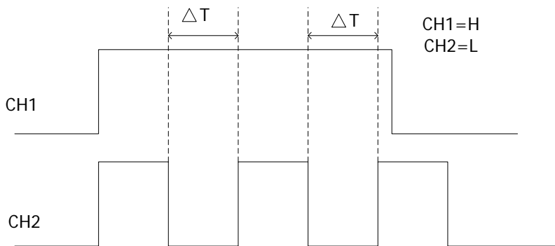
Figure 5-11 Duration Trigger
