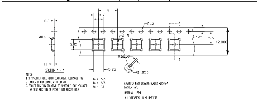
Figure 58. QFN32L (5x5x1) carrier tape outline
