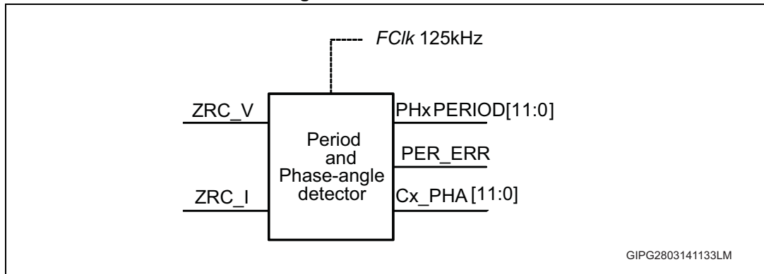
Figure 41. Phase meter
