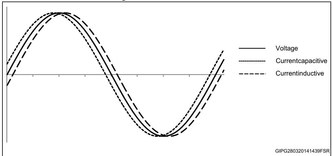
Figure 52. Phase shift error
