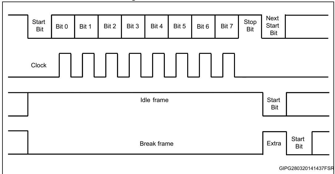
Figure 51. UART frame
