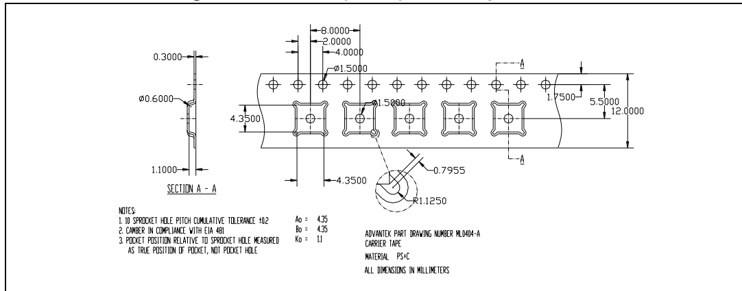
Figure 57. QFN24L (4x4x1) carrier tape outline
