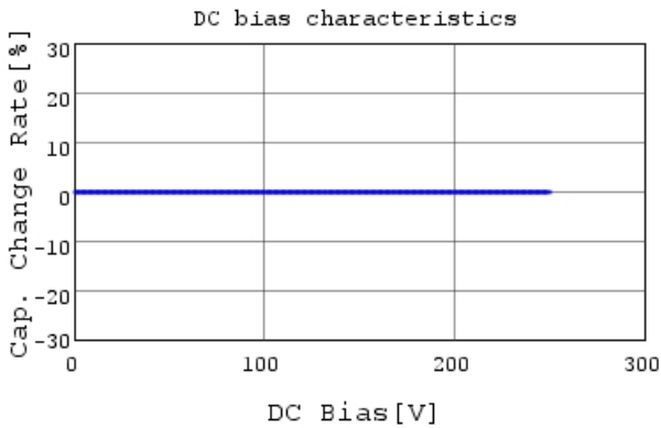
GRM21A5C2E330JW01 C-DC bias capchange, 25.0c
