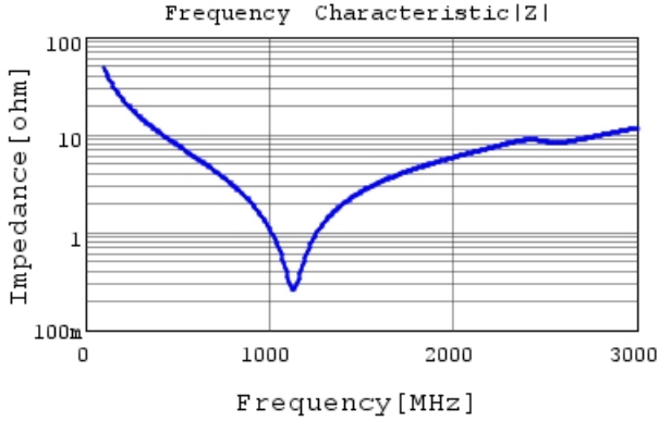
GRM21A5C2E330JW01 |Z| DCOV, 25degC
