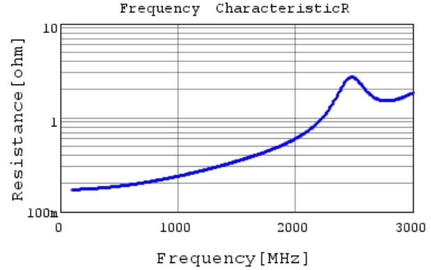
GRM21A5C2E330JW01 R DCOV, 25degC
