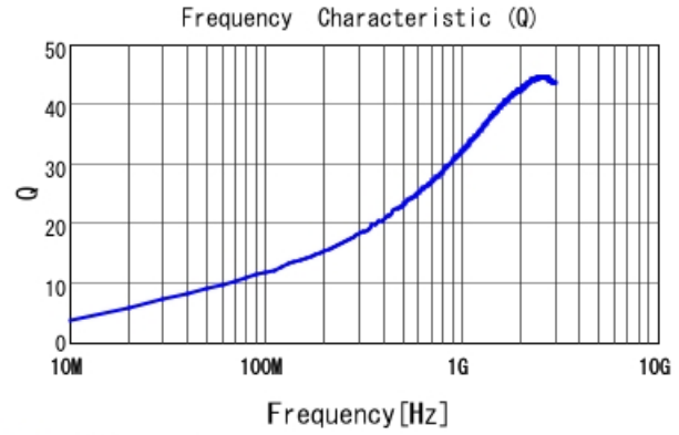
■ LQG15HS3N3S02 Q
