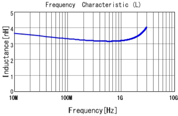
■ LQG15HS3N3S02 L
