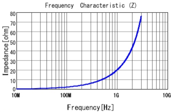
■ LQG15HS3N3S02 |Z|
