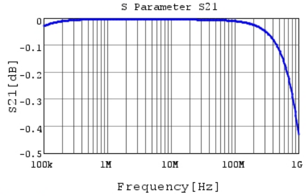
■ RDER71H224K1M1H03A S21 DC0V, 25degC
