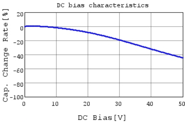
RDER71H224K1M1H03A C-DC bias capchange, 25.0
