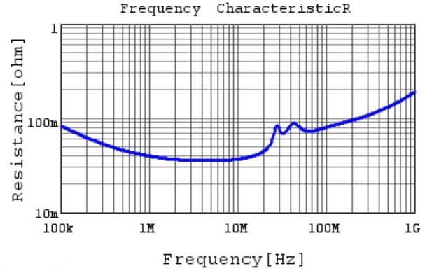
RDER71H224K1M1H03A R DCOV, 25degC
