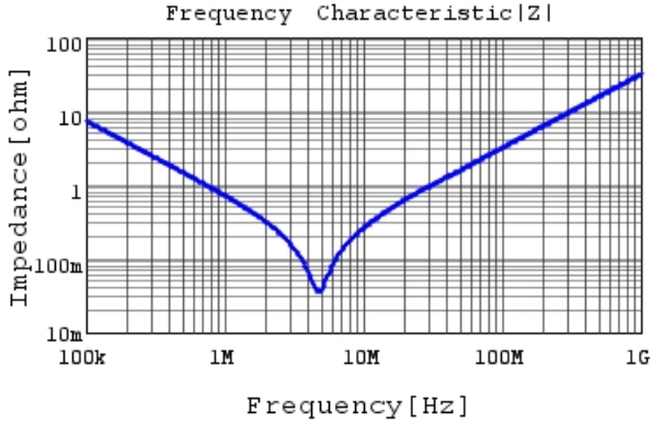
RDER71H224K1M1H03A |Z| DCOV, 25degC
