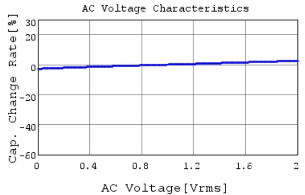
RDER71H224K1M1H03A C-AC Voltage capchange, I
