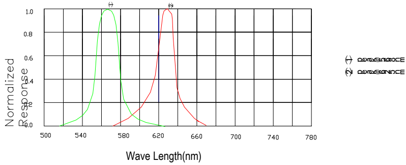
Spectral Reduance
