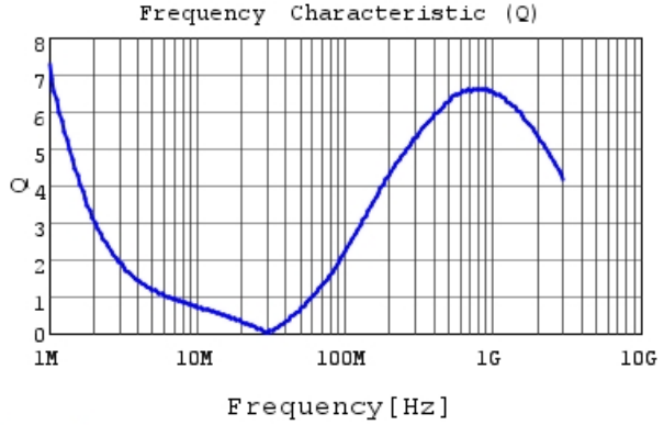
LQM21DN470N00 Q
