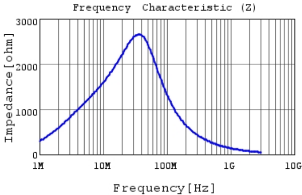
LQM21DN470N00 |Z|
