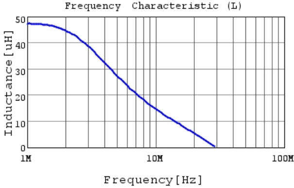
LQM21DN470N00 L
