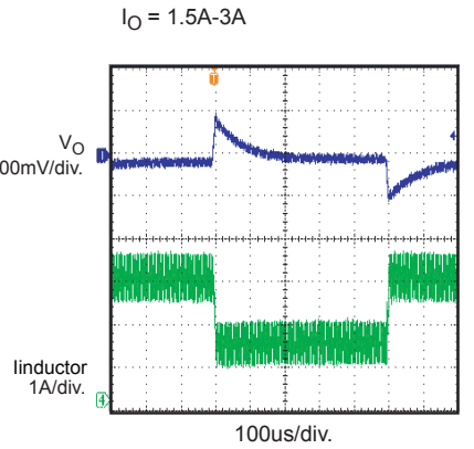
Loop Response
