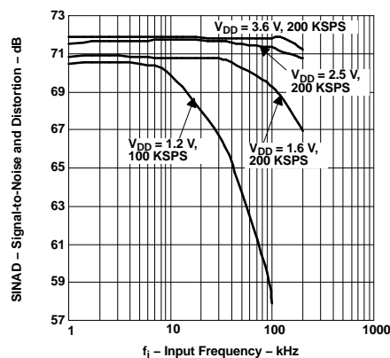
SIGNAL-TO-NOISE AND DISTORTION vs INPUT FREQUENCY
