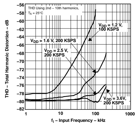
TOTAL HARMONIC DISTORTION vs INPUT FREQUENCY
