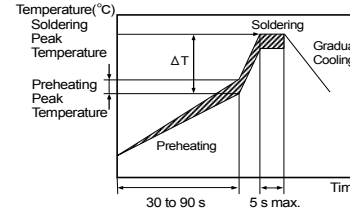
[Allowable Flow Soldering Temperature and Time]
