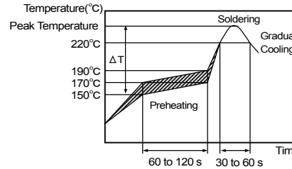
[Standard Conditions for Reflow Soldering]
