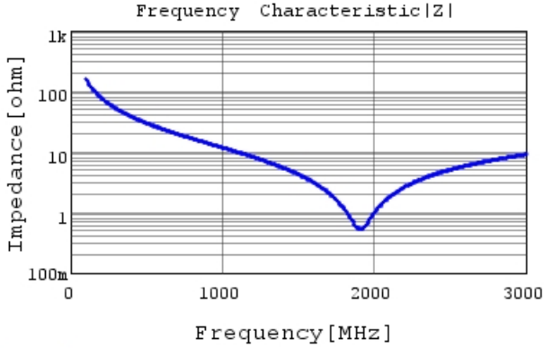
GRM21A5C2E100JW01 |Z| DCOV, 25degC
