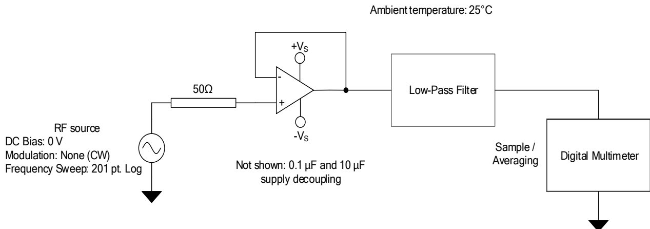
Figure 3. EMIRR IN+ Test Configuration Schematic
