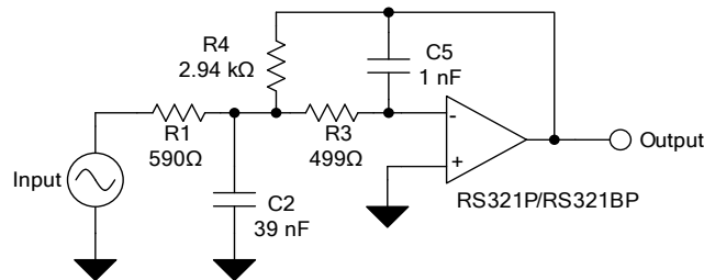
Figure 4. 25-kHz Low-Pass Filter
