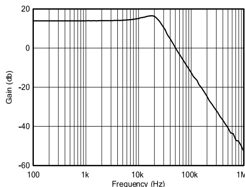
Figure 5. Low-pass filter transfer function
