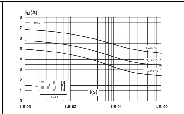
Figure 6. Non repetitive surge peak forward current versus overload duration (maximum values) (SMA)
