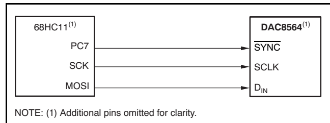
Figure 103. DAC8564 to 68HC11 Interface
