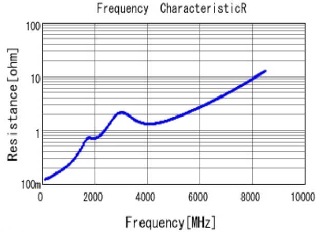
■ GRM1882C1H101JA01 R DCOV, 20degC
