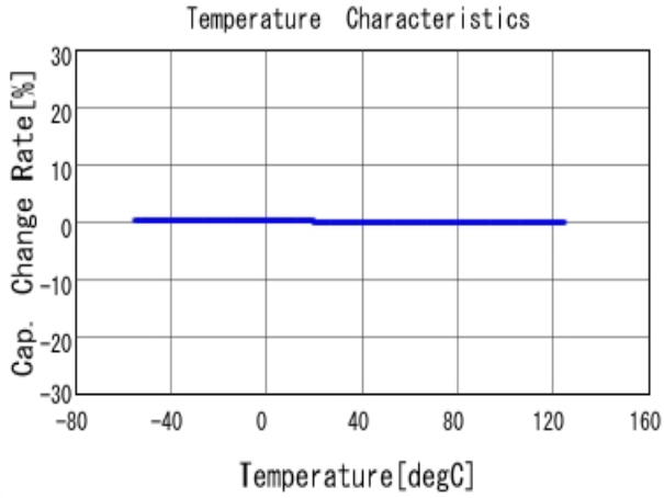
■ GRM1882C1H101JA01 C-Temp. capchange, DCOV, AC1Vrms
