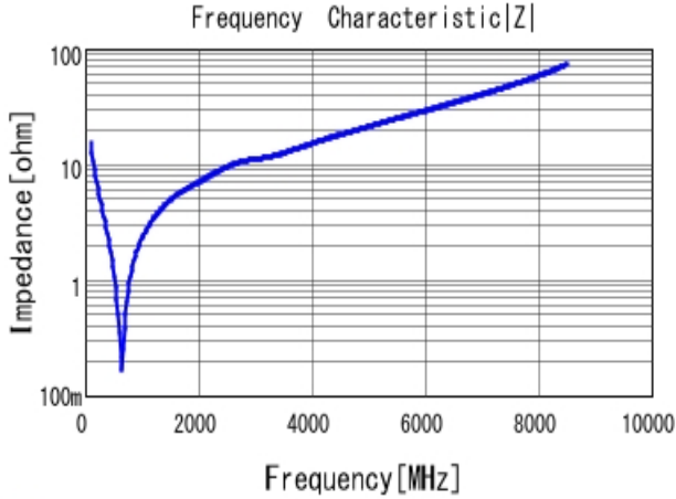
■ GRM1882C1H101JA01 |Z| DCOV, 20degC
