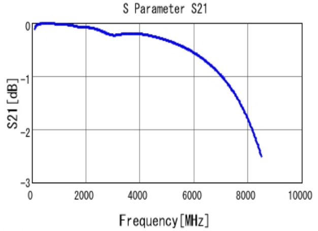
■ GRM1882C1H101JA01 S21 DCOV, 20degC
