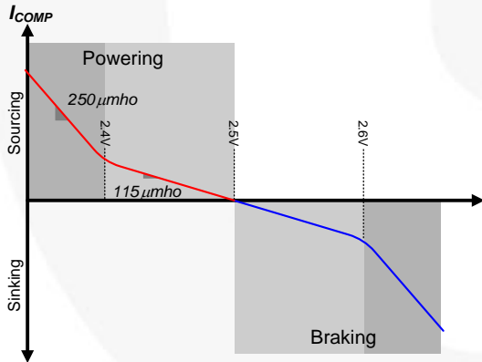
Figure 34. Gain Characteristic
