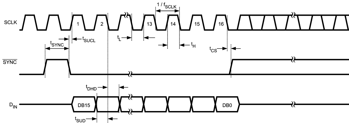
FIGURE 2. DAC121S101 Timing
