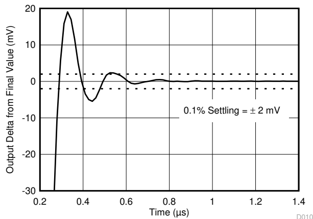
Figure 7-25. Large-Signal Step Response
