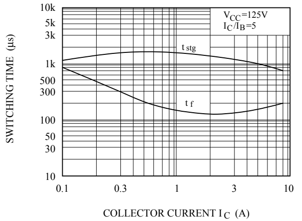
SWITCHING CHARACTERISTIC
