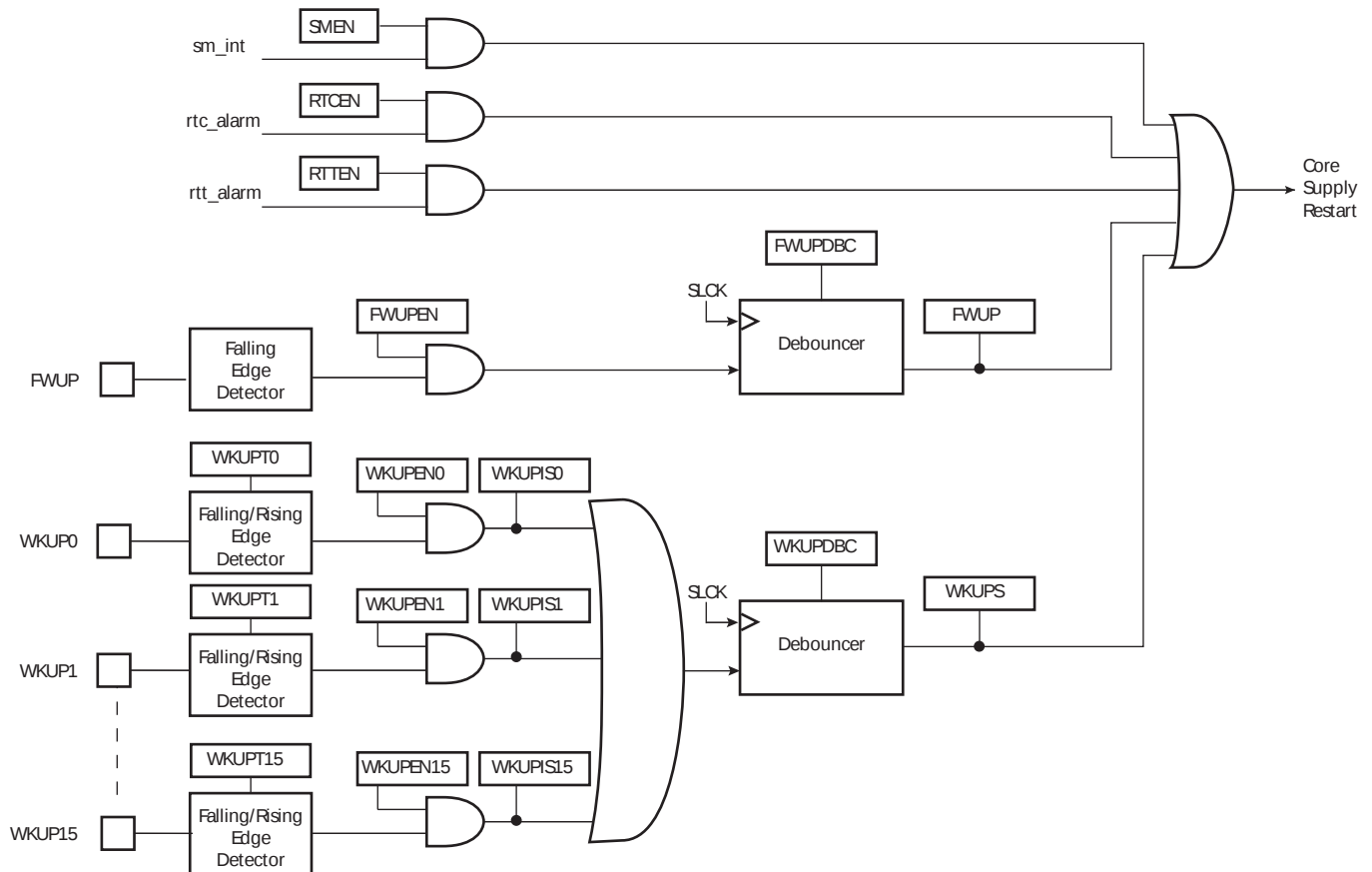
Figure 5-3. Wake-up Source
