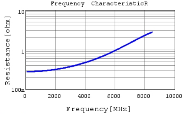
GRM1555C1H3R0BA01 R DCOV, 25degC
