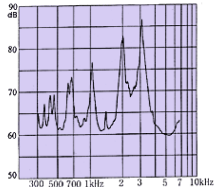
3VP-P Square Wave/10cm
