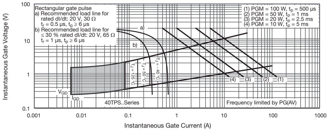
Fig. 8 - Gate Characteristics
