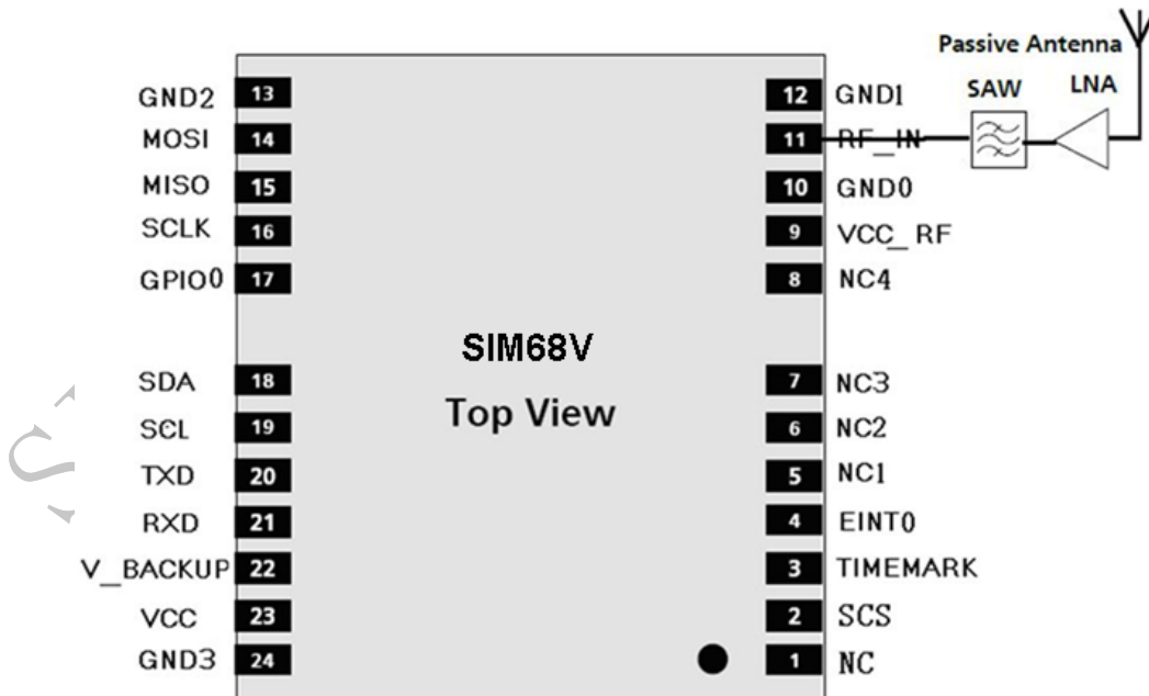
Figure 7: SIM68V passive antenna design (with external LNA and SAW)
