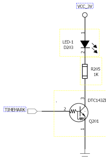
Figure 5: TIMEMARK application circuit
