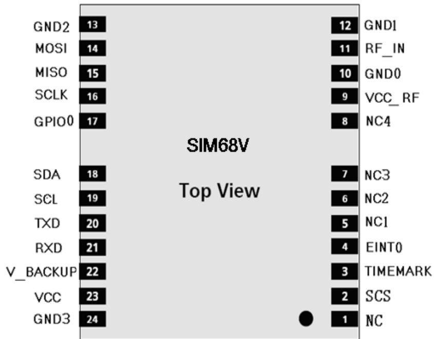
Figure 2: SIM68V pin out diagram (Top view)
