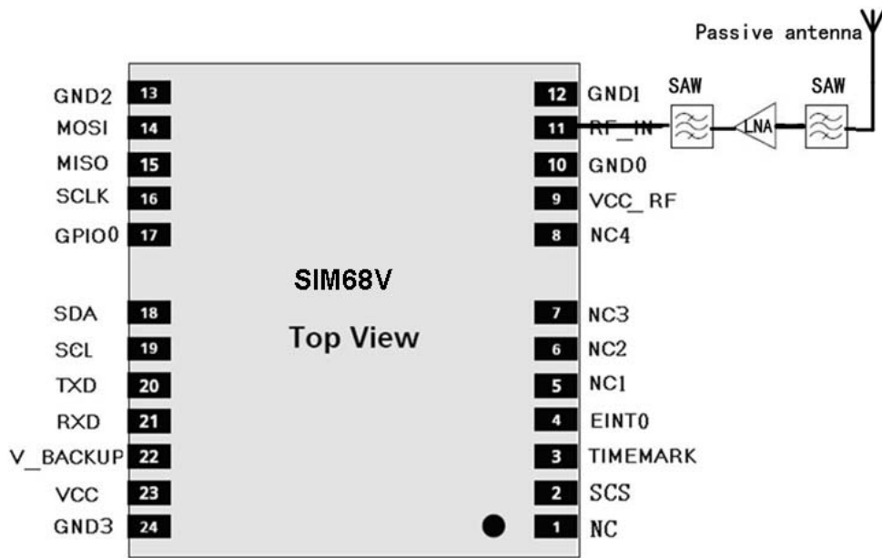
Figure 8: SIM68V passive antenna design for best performance and increased immunity
