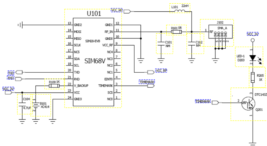
Figure 13: Example application schematic with UART
