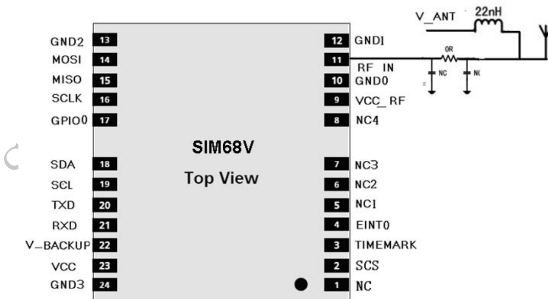
Figure 9: SIM68V active antenna design
