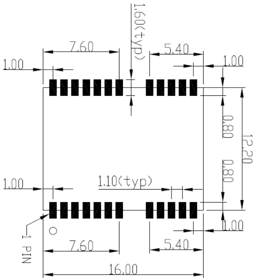
Figure 4: Recommended PCB decal (top view) (Unit: mm)
