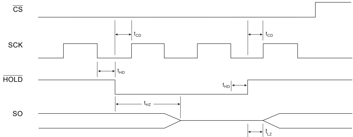
Figure 5-3. Hold Timing
