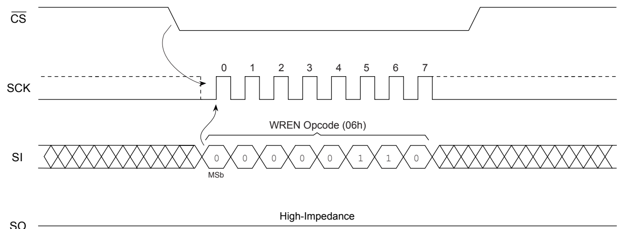
Figure 6-2. WREN Timing
