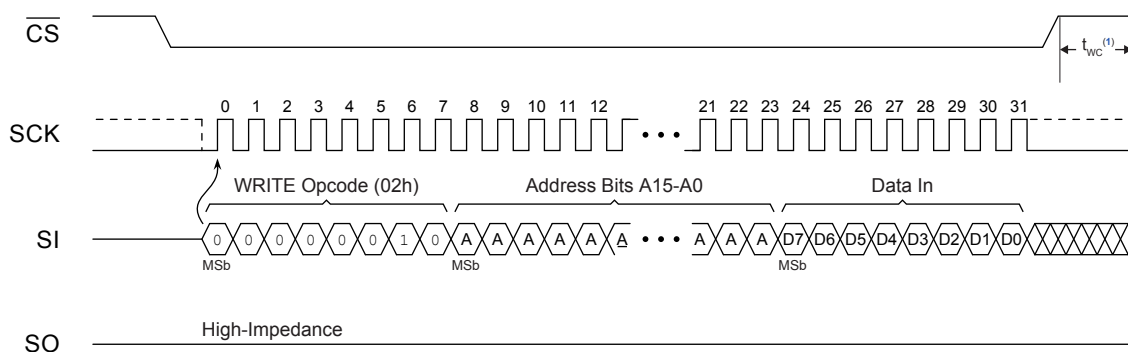
Figure 8-1. Byte Write
