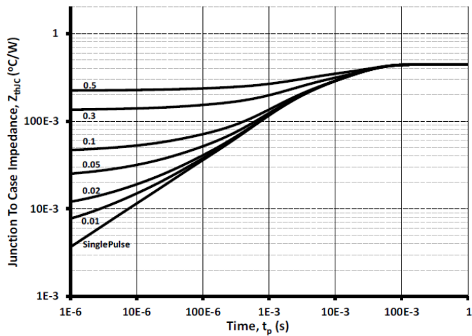
Figure 19. Transient thermal impedance (junction - case)
