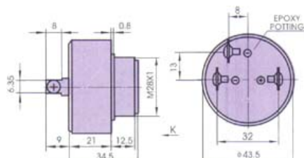
PIN(P) TYPE
