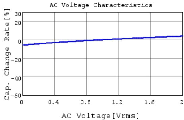
GRM32EC72A106KE05 C-AC Voltage capchange, Dc
