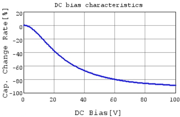
GRM32EC72A106KE05 C-DC bias capchange, 25.0c
