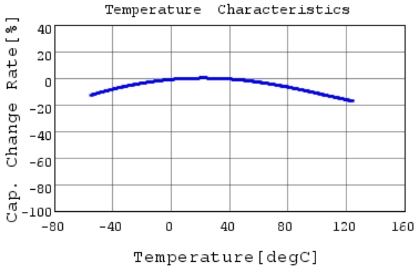
GRM32EC72A106KE05 C-Temp. capchange, DC0.0V,
