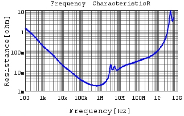
GRM32EC72A106KE05 R DCOV, 25degC
