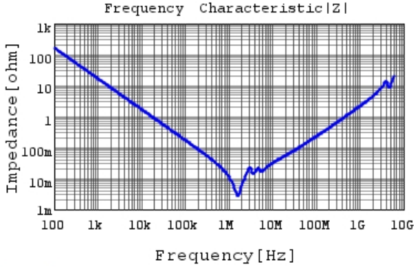
GRM32EC72A106KE05 |Z| DCOV, 25degC
