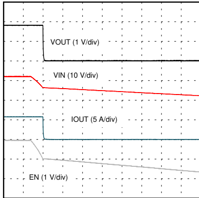
Figure 8-20. V_{IN} Shutdown
