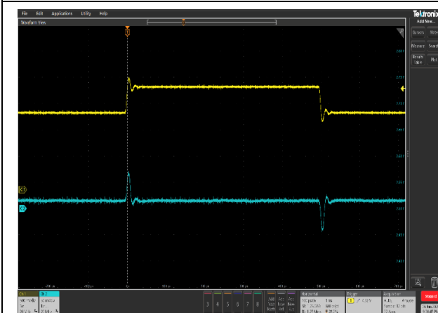
Figure 15. Line Transient, 500 mV Step, C_{\text{IN}} = 1\ \mu\text{F} , C_{\text{OUT}} = 1\ \mu\text{F} , 50 mV/div
