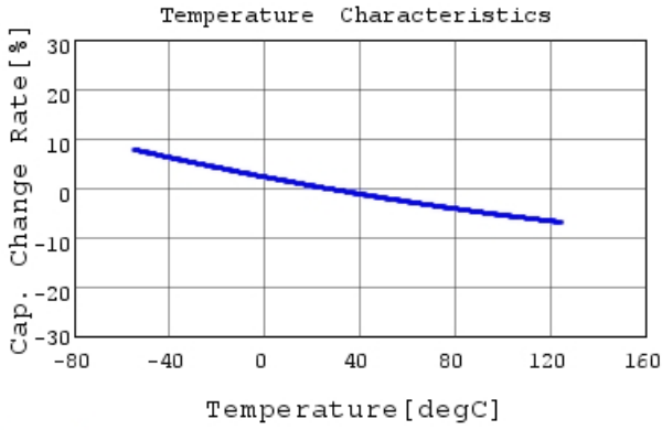
GRM2167U1H153JA01 C-Temp. capchange, DCOV, 1
