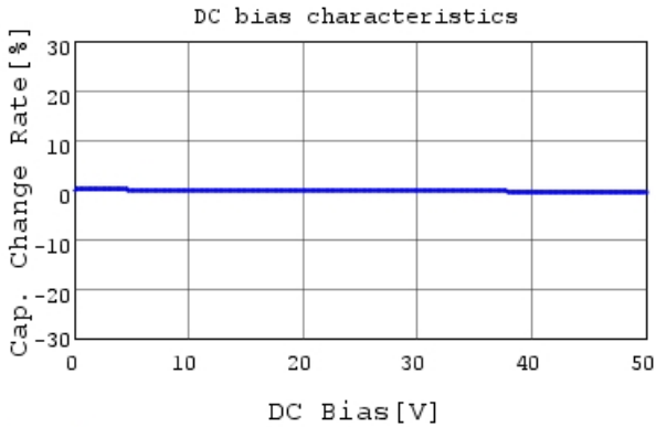
GRM2167U1H153JA01 C-DC bias capchange, 25.0c
