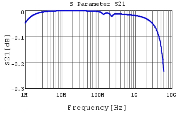
GRM2167U1H153JA01 S21 DCOV, 25degC
