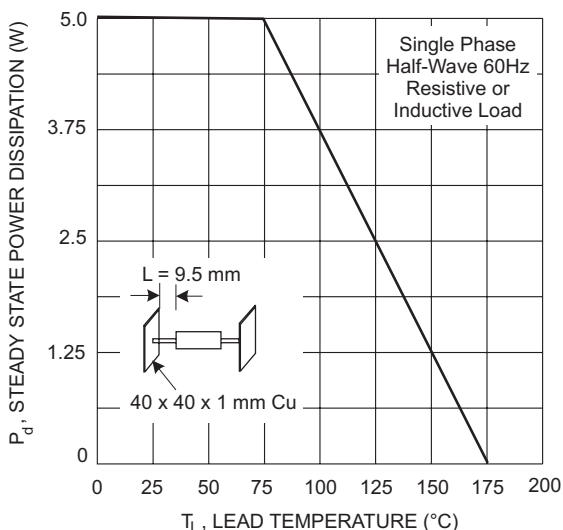
Fig. 5, Steady State Power Derating
