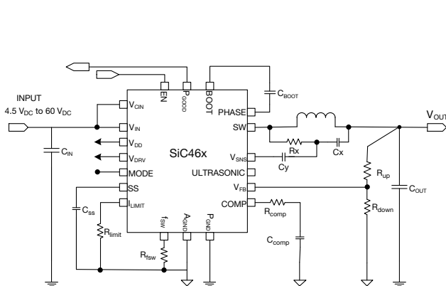
Fig. 1 - Typical Application Circuit for SiC46x
