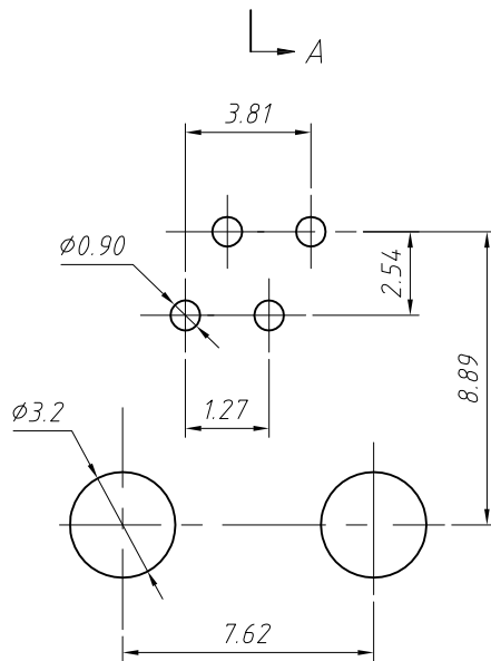
PCB Layout
