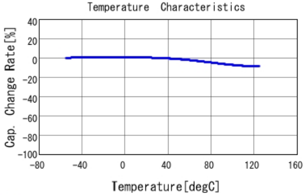
■ KRM55QR72A106KH01 C-Temp. capchange, DCOV, AC1Vrms
