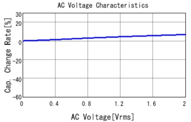
■ KRM55QR72A106KH01 C-AC Voltage capchange, DCOV, 25.0d
