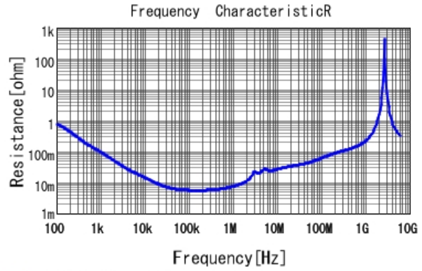
■ KRM55QR72A106KH01 R DCOV, 25degC
