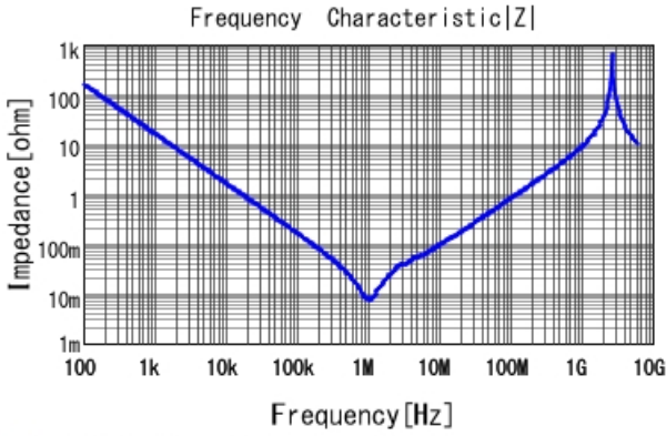
■ KRM55QR72A106KH01 |Z| DCOV, 25degC
