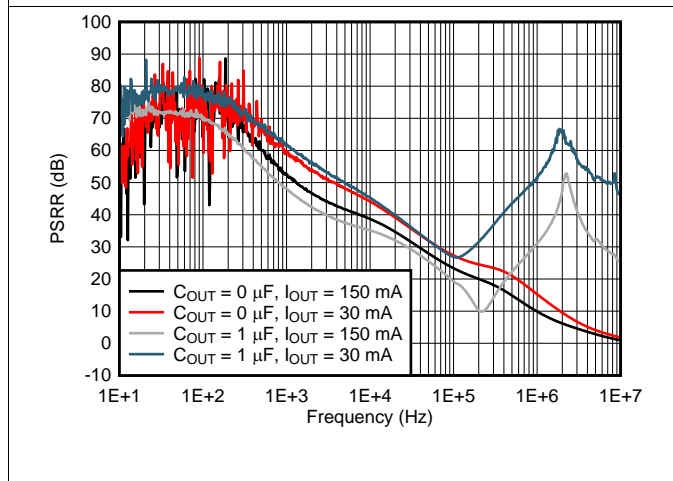
Figure 9. Power-Supply Rejection Ratio Over C_{OUT}
