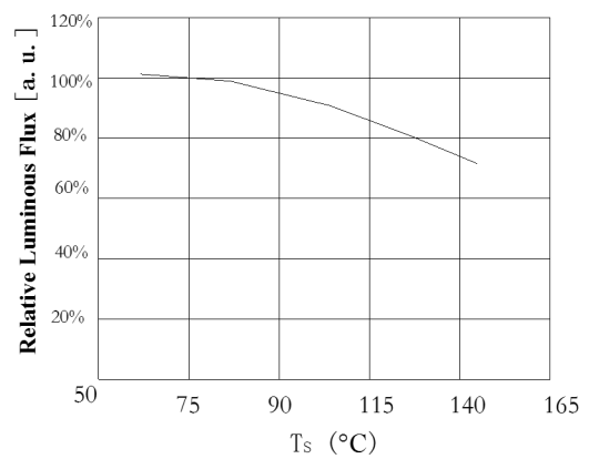
Case Temperature vs. Relative Luminous Flux 结点温度与相对流明曲线图 IF=1440mA
