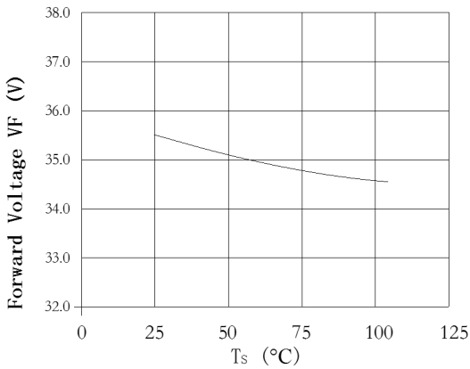
Case Temperature vs. Forward Voltage 结点温度与正向电压曲线图 IF=1440mA
