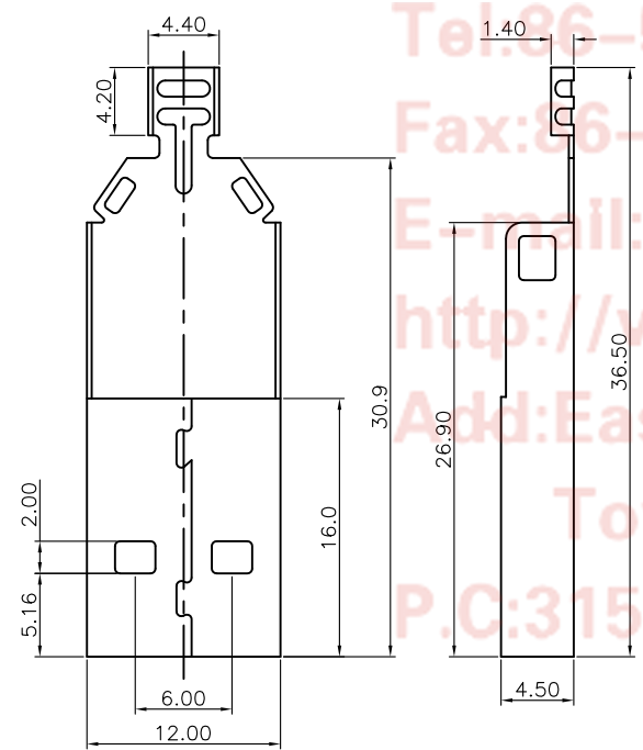
Down shell
