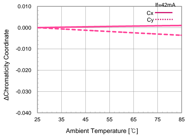
▪ Chromaticity Coordinate vs. Temperature
