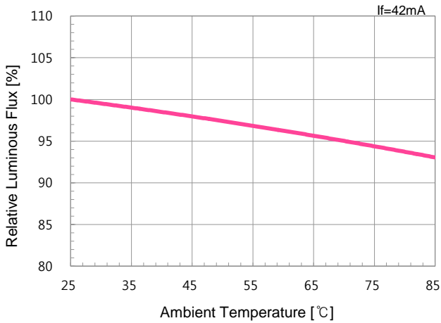
▪ Luminous Flux vs. Temperature
