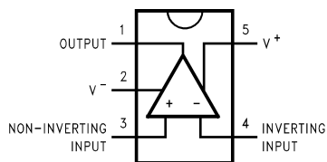
Figure 3. Top View
